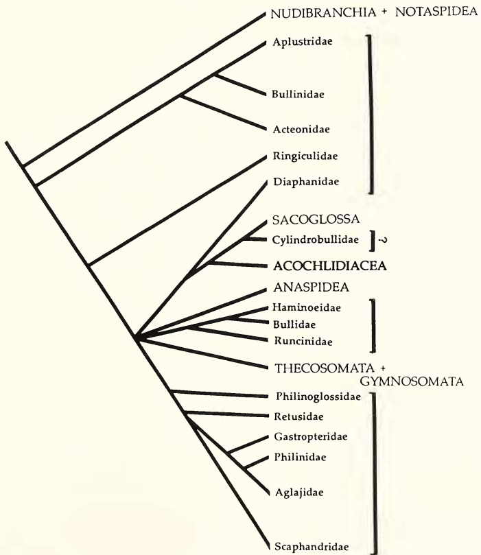
Figure 5. GOSLINER's (1978: pl. 22, fig. 36) phylogeny of the Opisthobranchia, redrawn as a modern cladogram. Solid horizontal bar denotes present Cephalaspidia.
